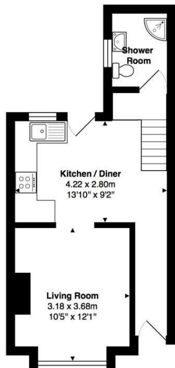
Ground Floor Area: 31.3 m 2 ... 337 ft 2
